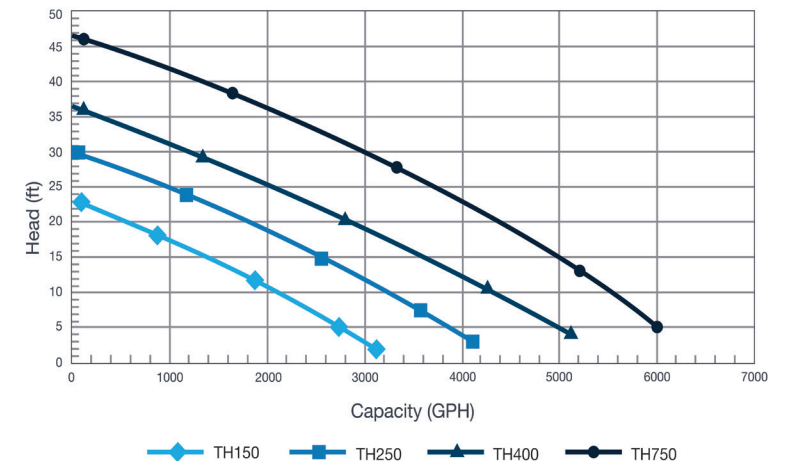
EasyPro TH Pump Performance
