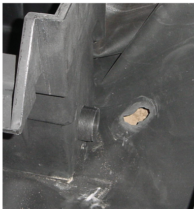
Hold bulkhead up to spillway and cut hole in liner just smaller than bulkhead.
