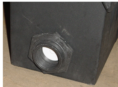
Bulkhead fitting and plug installed in the end of the spillway
